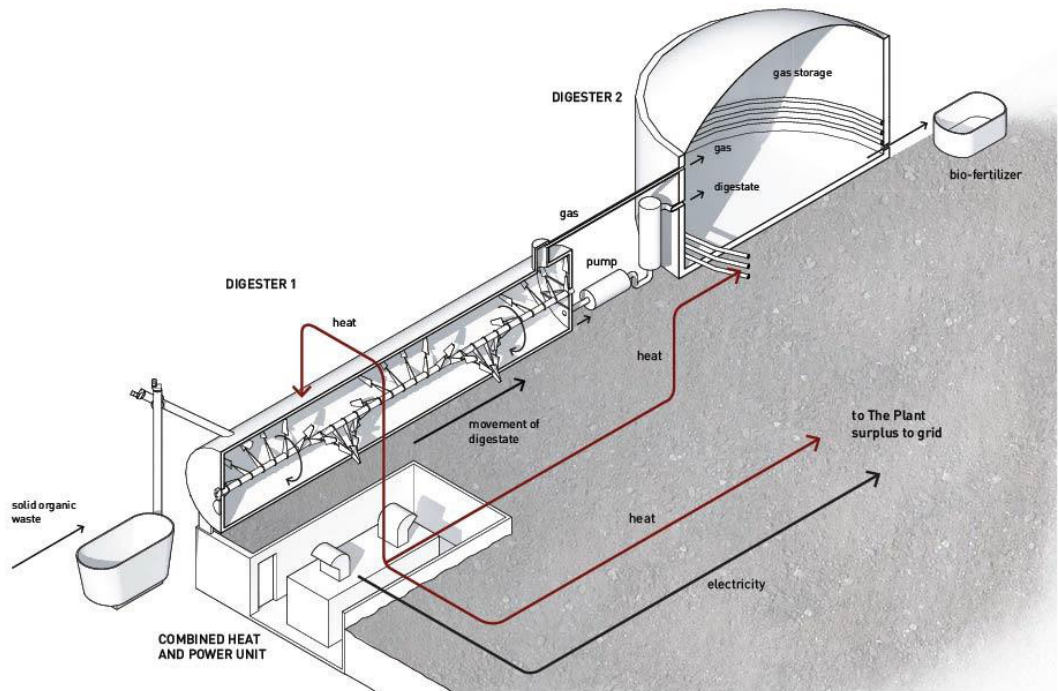
Figure 3: The Plant Chicago Anaerobic Digester and System Integration Diagram, Creating Urban Agricultural Systems (Proksch 2017)
